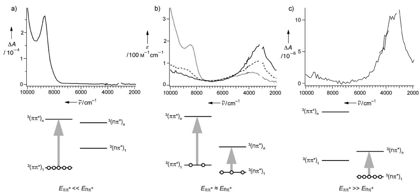
Figure 2. Time-resolved near-infrared spectra at 0–1 \mu s (upper part) and energy diagrams with transitions corresponding to the bands observed in the spectra (lower) for a) AN, b) AP (—), Me-AP (---), and MeO-AP (----), and c) CF 3 -AP.
